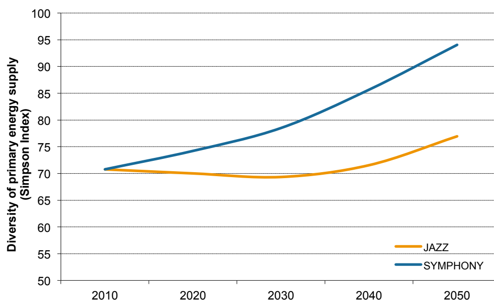
Figure 84 – Diversity of primary energy supply (Simpson Index)
